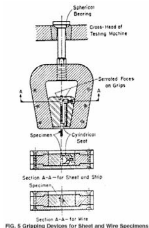
FIG. 5 Gripping Devices for Sheet and Wire Specimens
