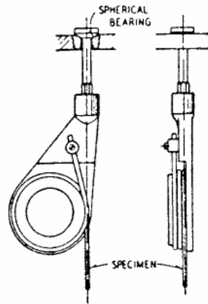
FIG. 6 Snubbing Device for Testing Wire
